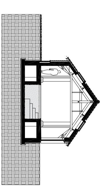
Section E - E Indoor swimming pool and wellness area
