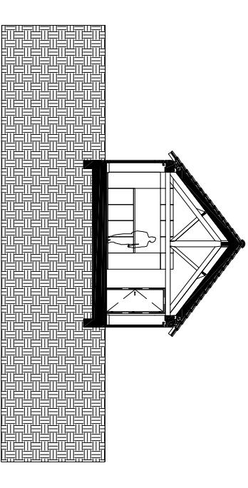
Section F - F Original building
