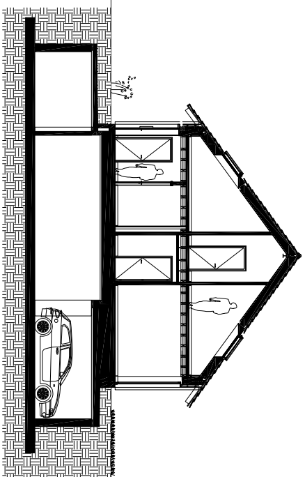
Section G - G Rebuilt building
