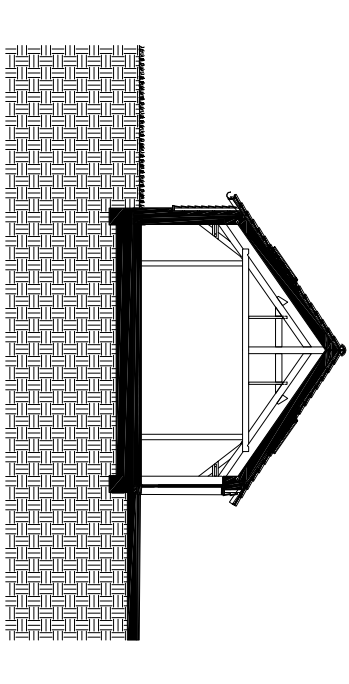
Section D - D Original building
